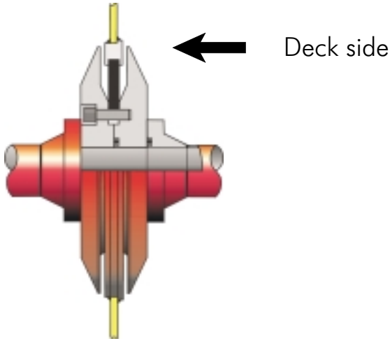
Resilient bulkhead penetration
